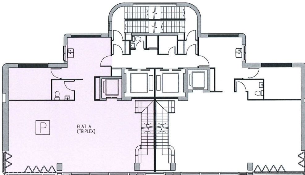
B/F, G/F, 1/F & 2/F FLAT A (TRIPLEX)
